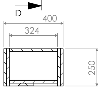
SECTION C-C SCALE 1 : 15
